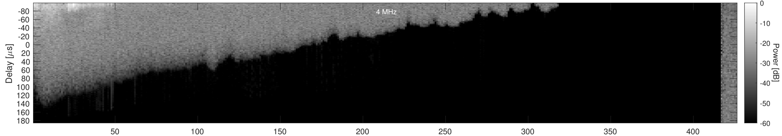
Orbit 5382, Window, Channel 2, Optimized
