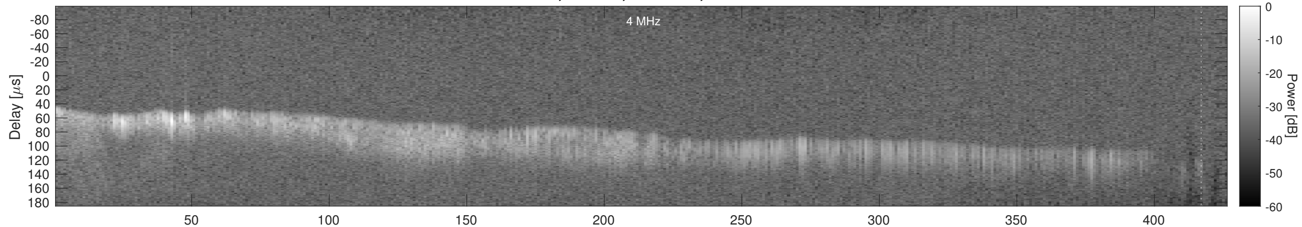
Orbit 5382, Window, Channel 2, Chapman
