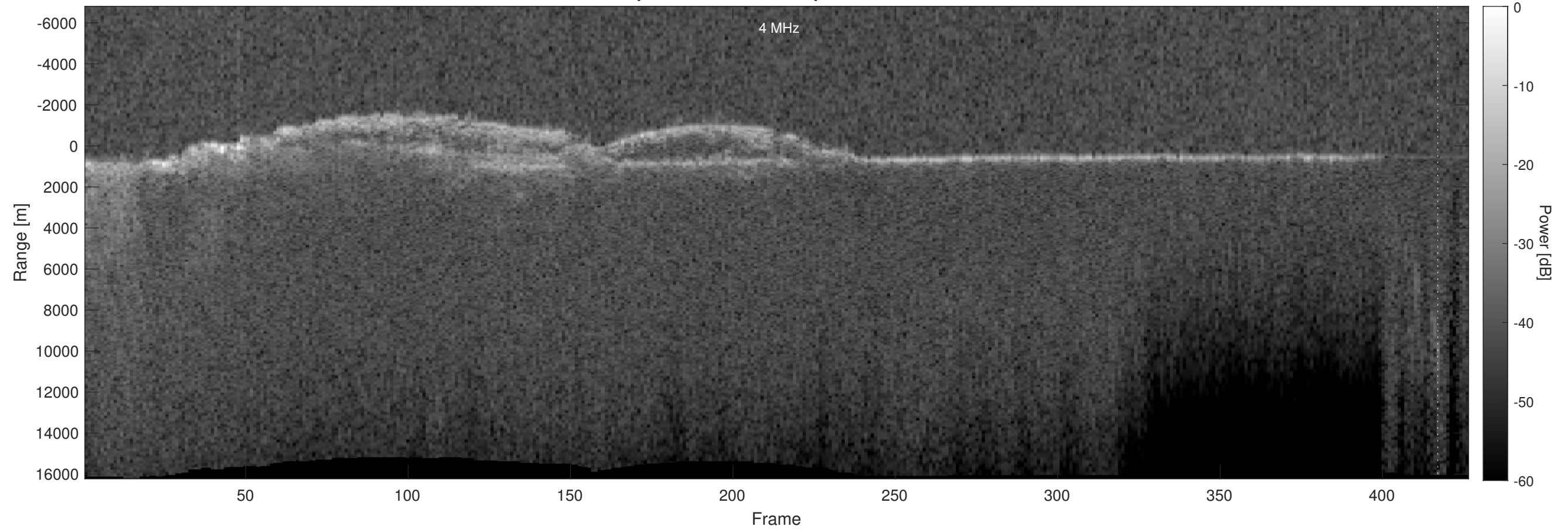
Orbit 5382, Optimized, Window, Depth-Corrected, Channel 2
