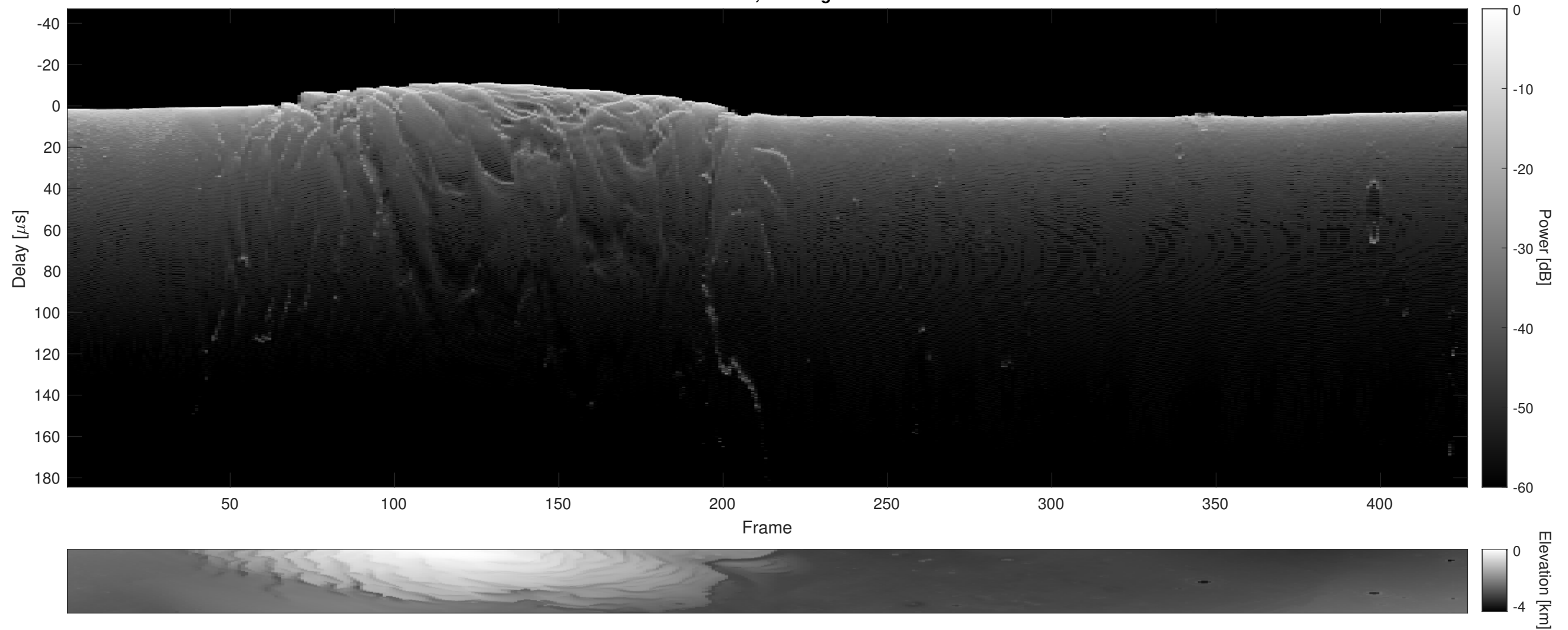
Orbit 5383, Cluttergram
