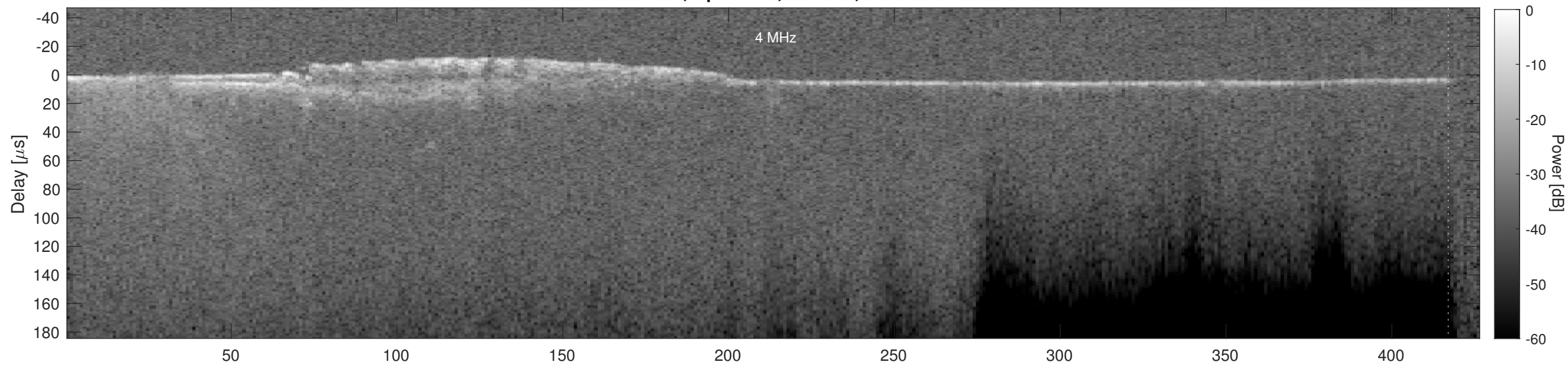
Orbit 5383, Cluttergram
