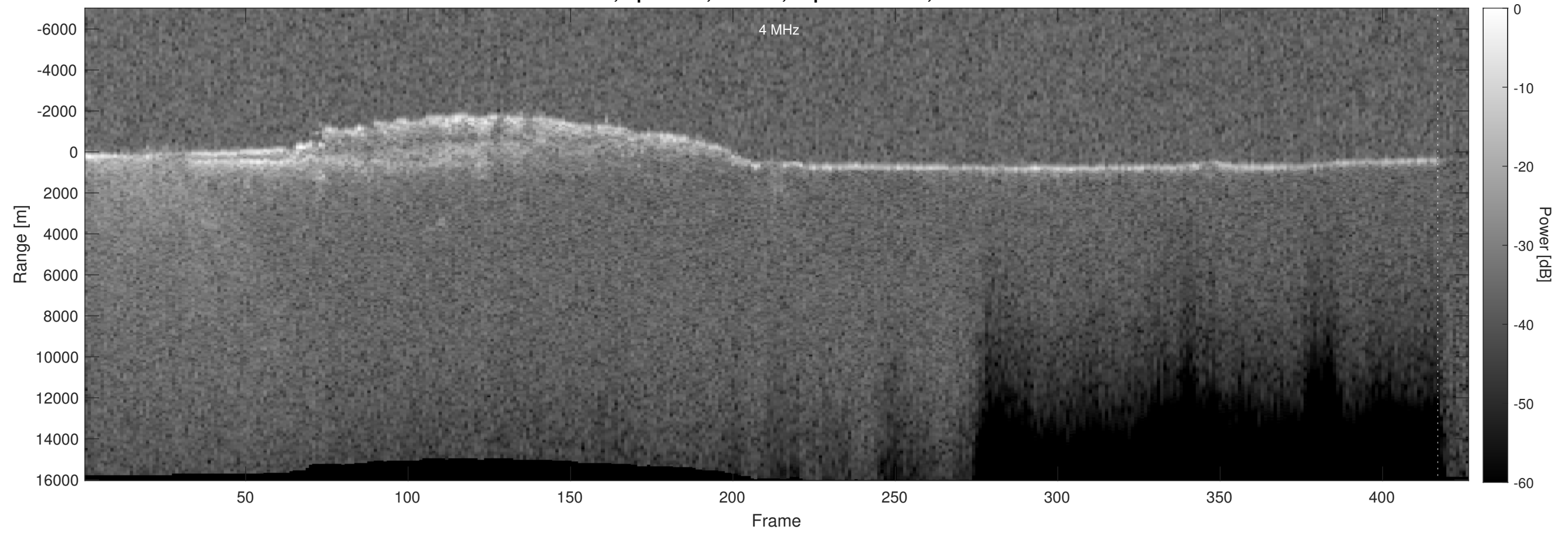
Orbit 5383, Optimized, Window, Depth-Corrected, Channel 2
