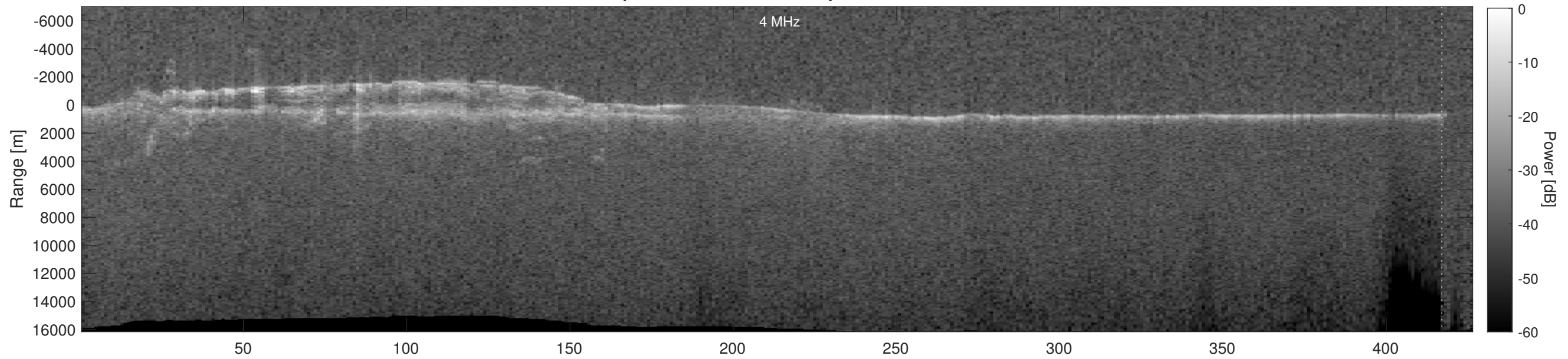
Orbit 5384, Depth-Corrected Cluttergram
