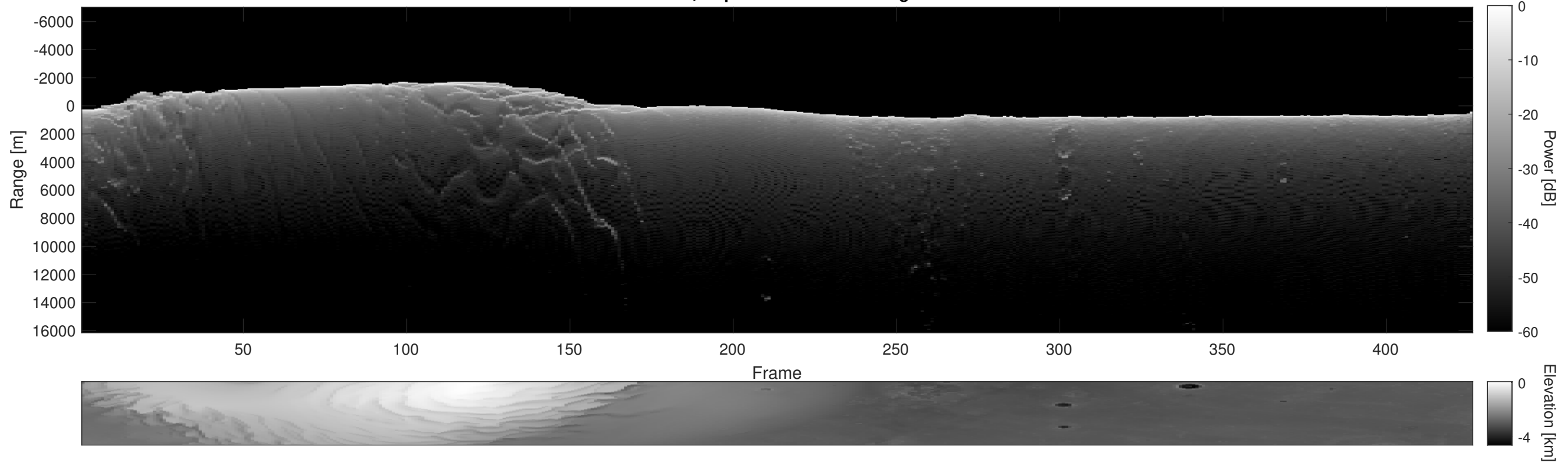
Orbit 5384, Depth-Corrected Cluttergram
