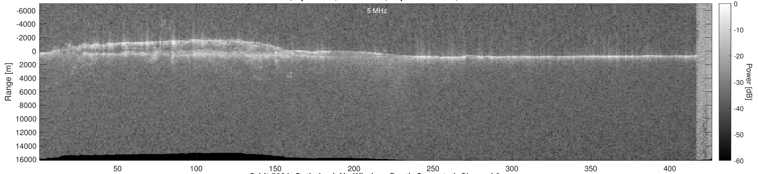
Orbit 5384, Optimized, No Window, Depth-Corrected, Channel 2
