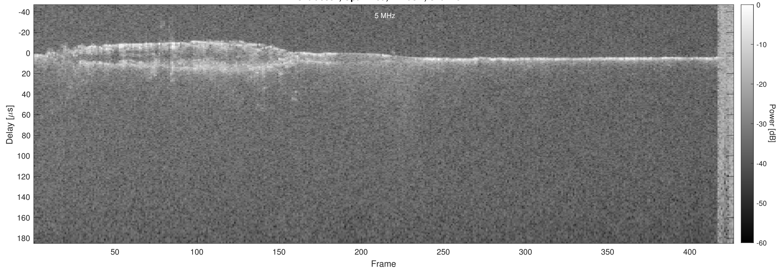
Orbit 5384, Optimized, Window, Channel 2
