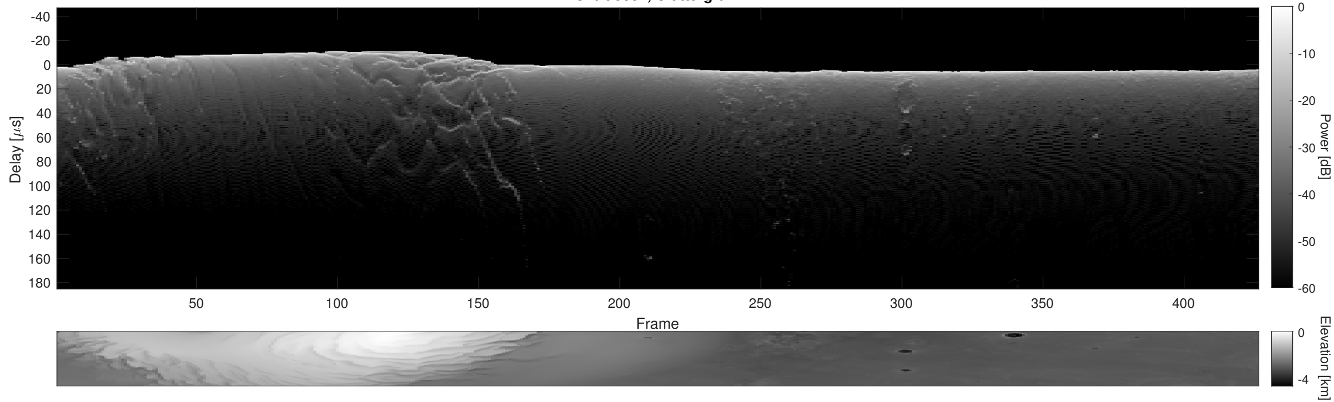
Orbit 5384, Cluttergram
