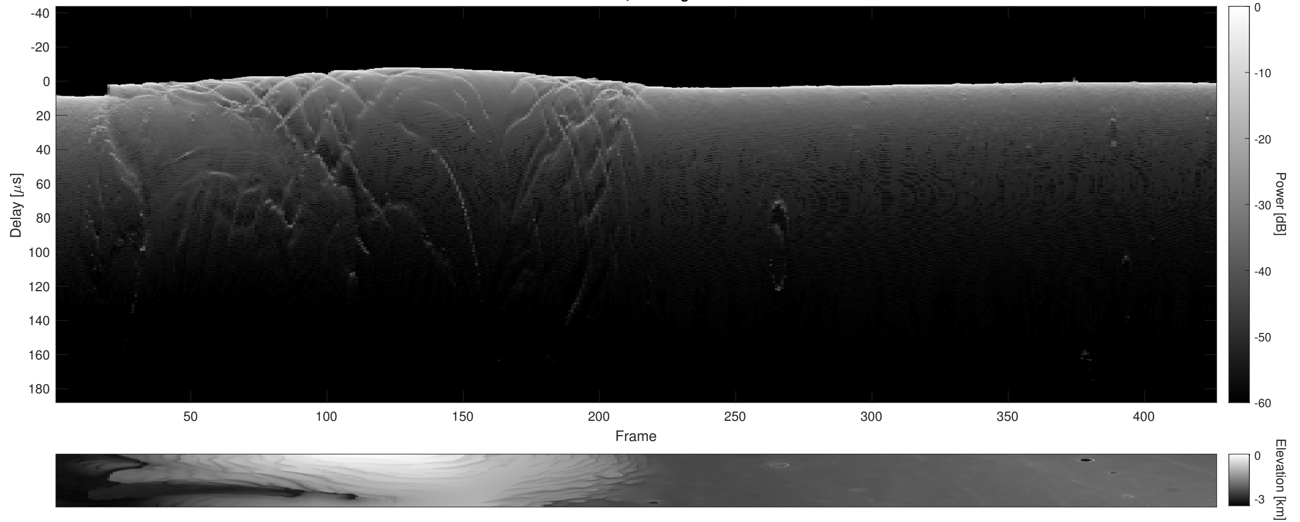
Orbit 5385, Cluttergram
