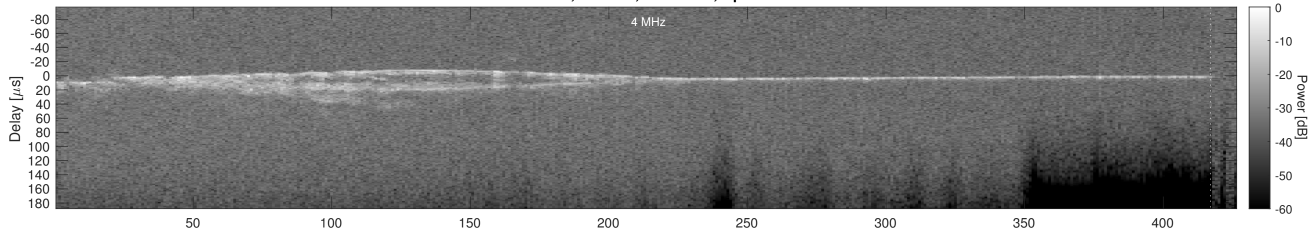
Orbit 5385, Cluttergram
