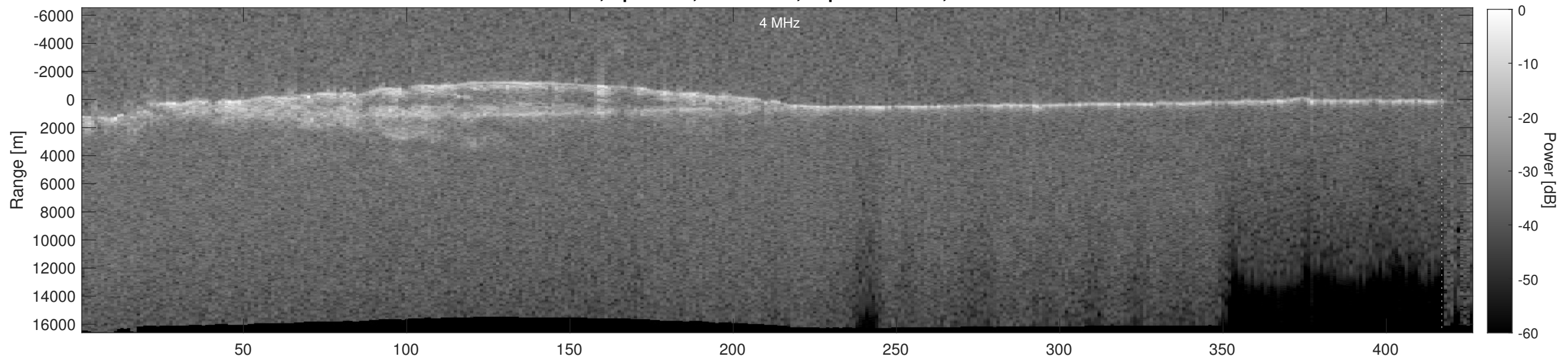
Orbit 5385, Depth-Corrected Cluttergram
