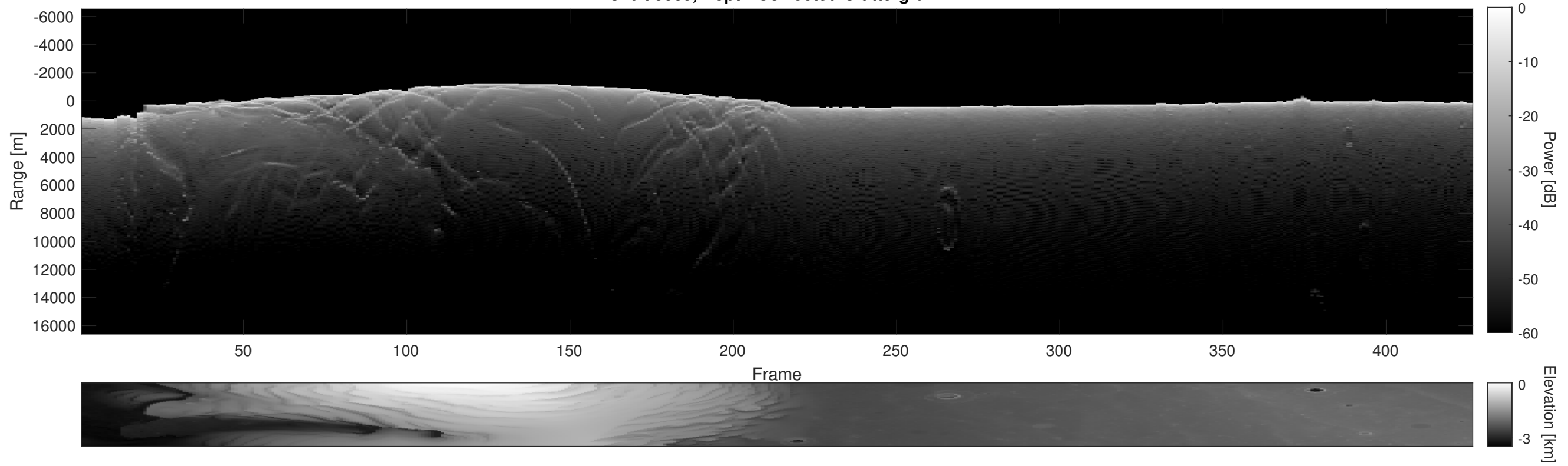
Orbit 5385, Depth-Corrected Cluttergram
