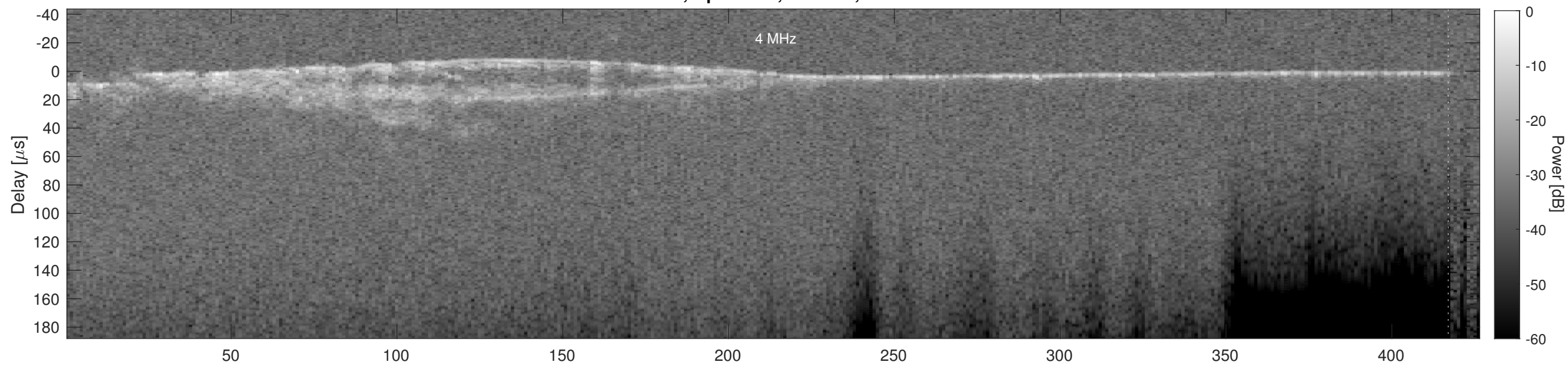
Orbit 5385, Cluttergram
