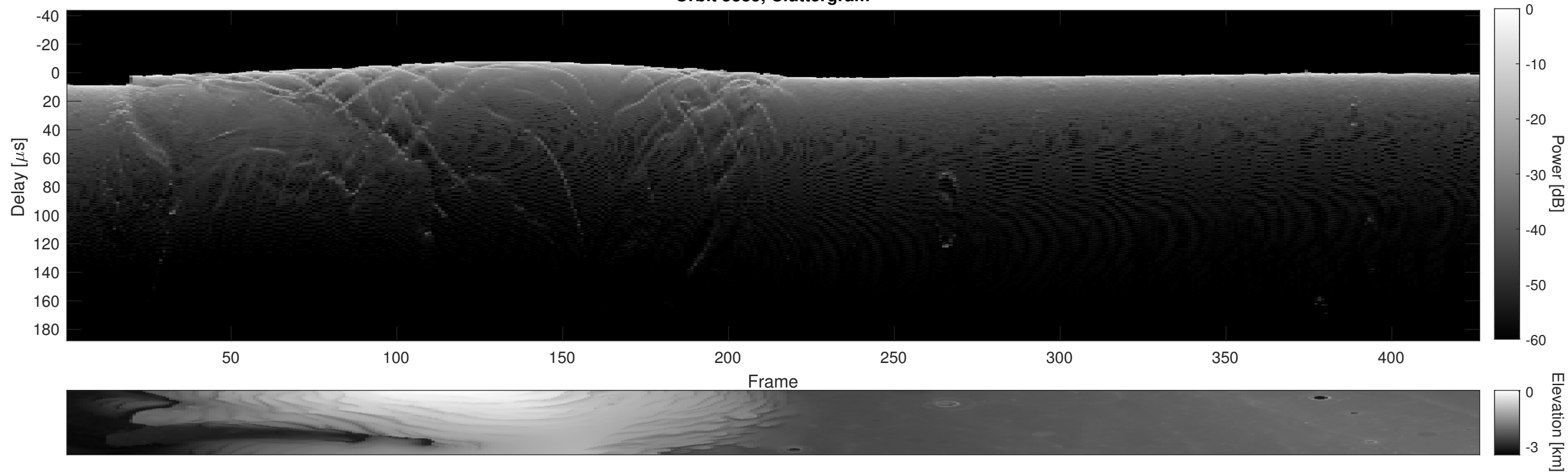
Orbit 5385, Cluttergram
