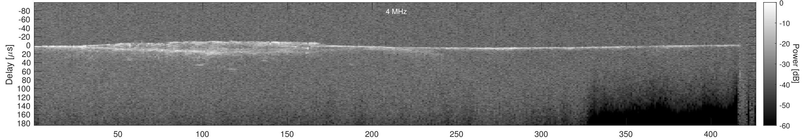
Orbit 5387, Cluttergram
