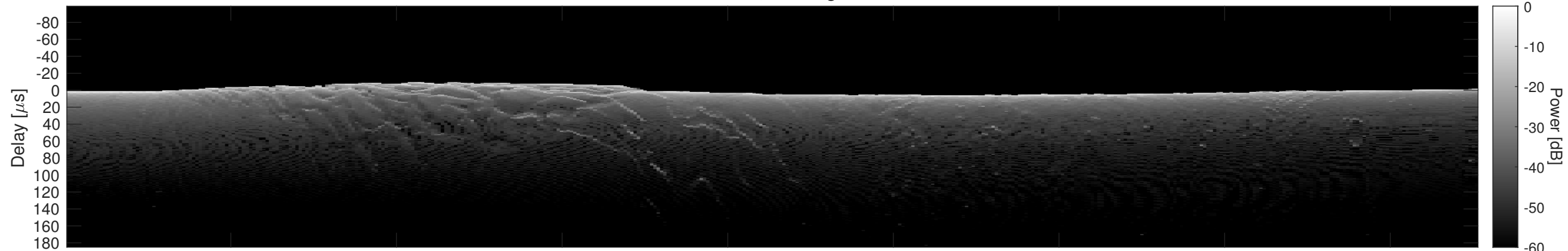
Orbit 5387, Cluttergram
