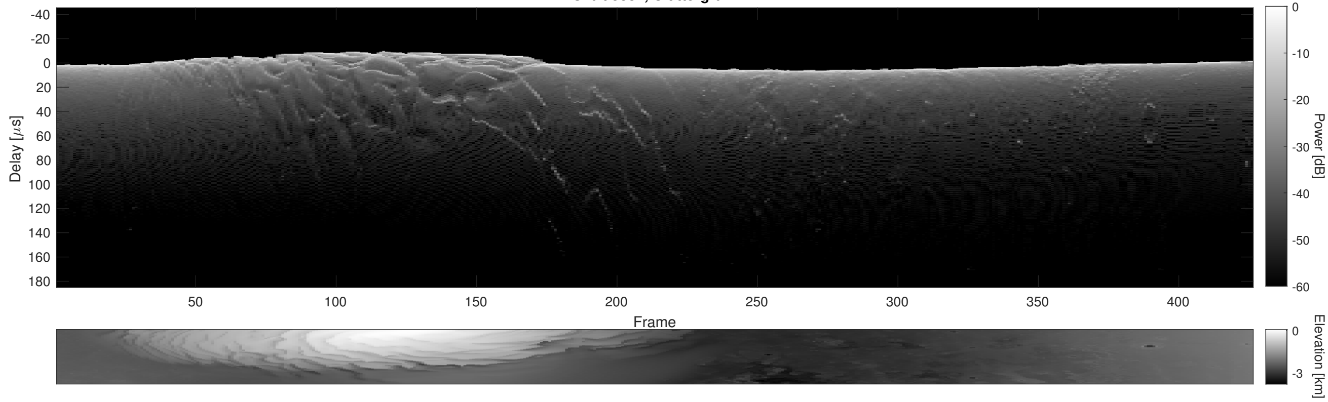
Orbit 5387, Cluttergram
