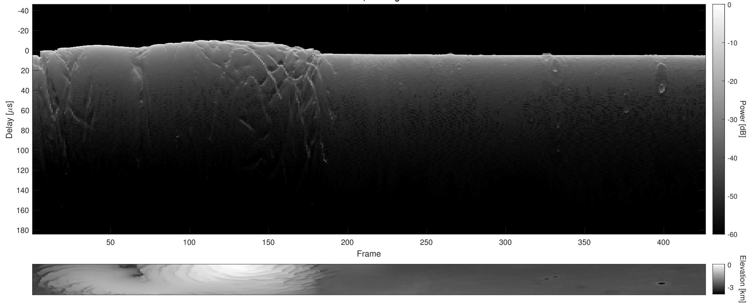
Orbit 5388, Cluttergram
