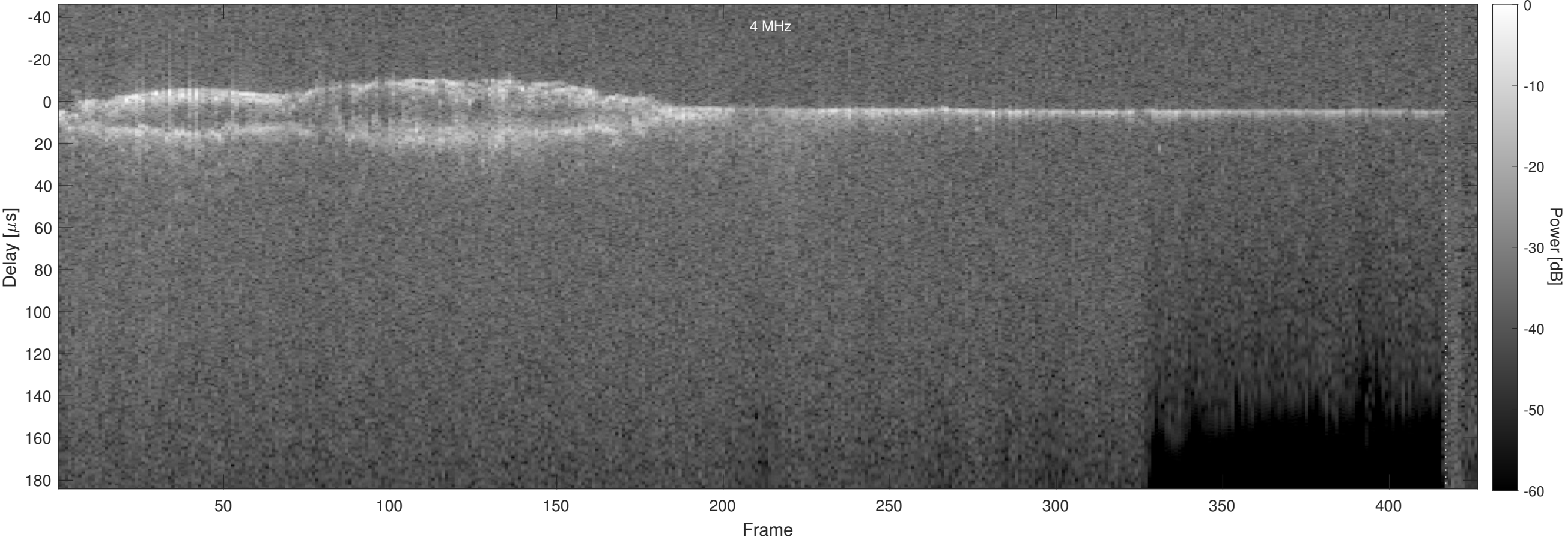
Orbit 5388, Optimized, No Window, Channel 2
