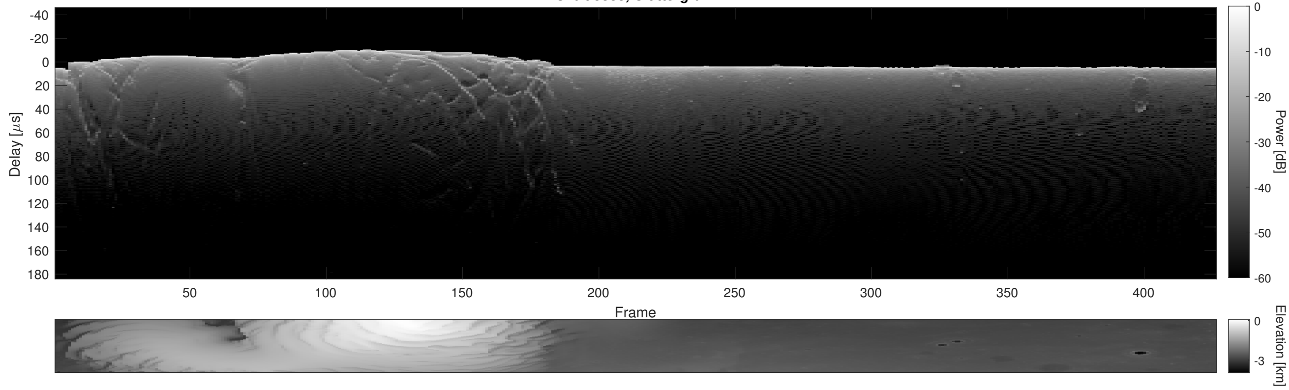
Orbit 5388, Cluttergram
