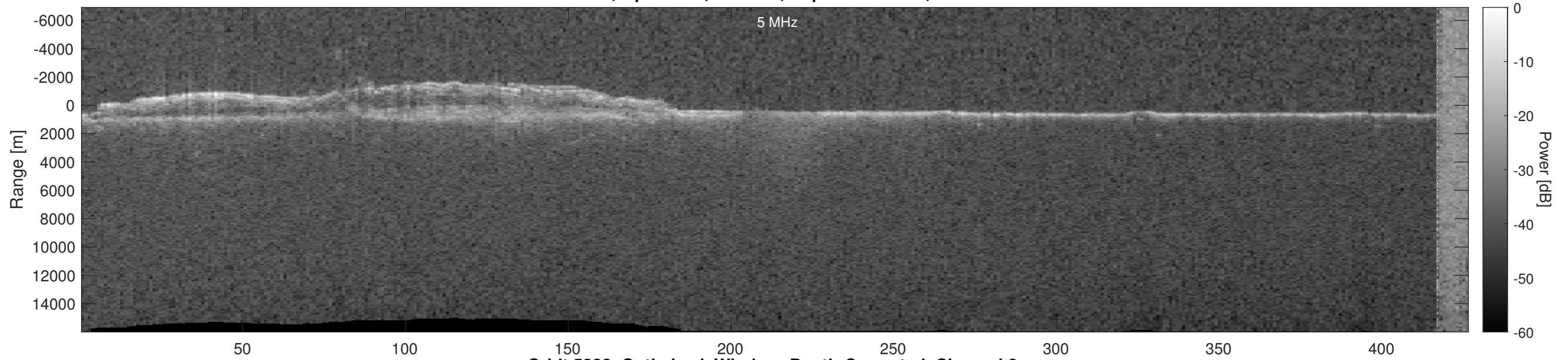
Orbit 5388, Optimized, Window, Depth-Corrected, Channel 2
