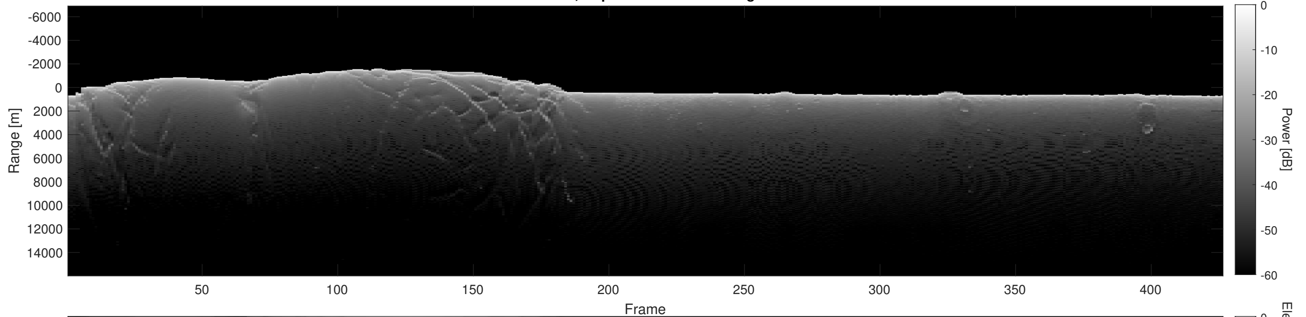
Orbit 5388, Depth-Corrected Cluttergram
