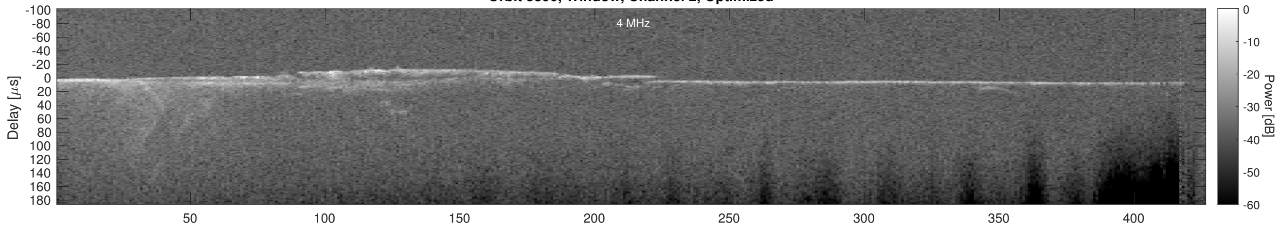
Orbit 5390, Cluttergram
