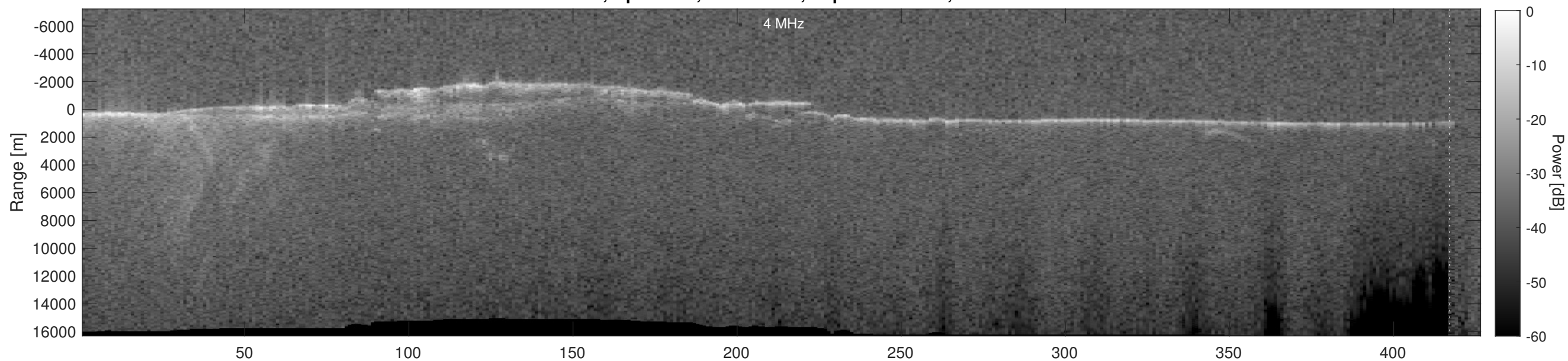
Orbit 5390, Depth-Corrected Cluttergram
