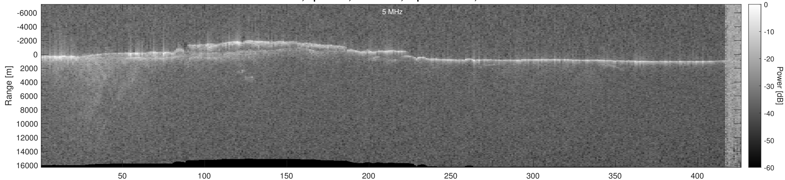
Orbit 5390, Optimized, No Window, Depth-Corrected, Channel 2
