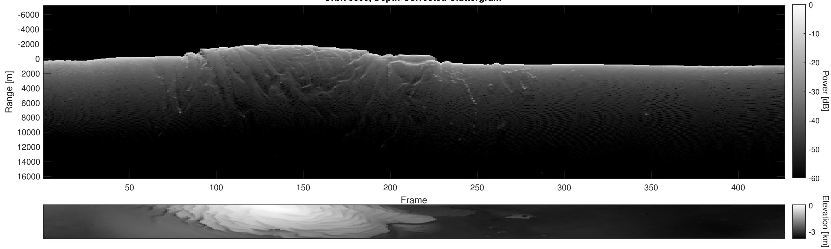
Orbit 5390, Depth-Corrected Cluttergram
