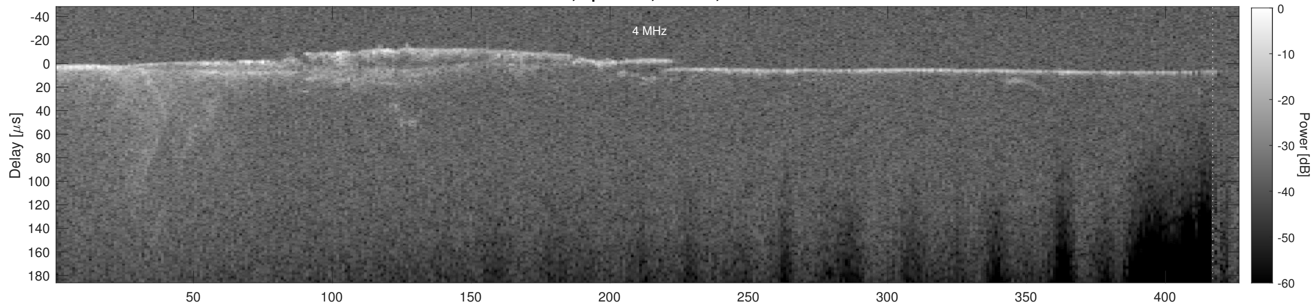
Orbit 5390, Cluttergram
