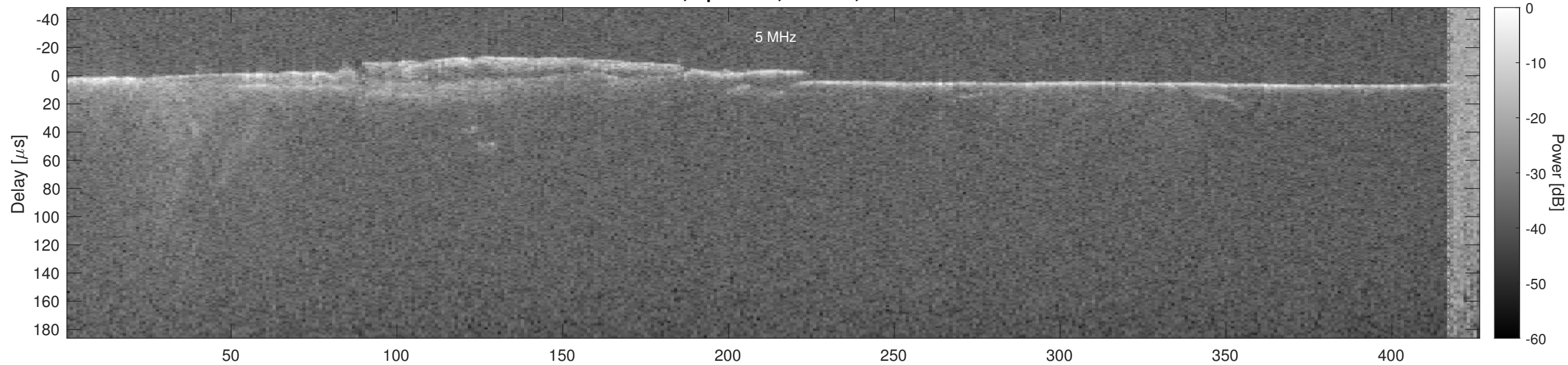
Orbit 5390, Optimized, Window, Channel 2
