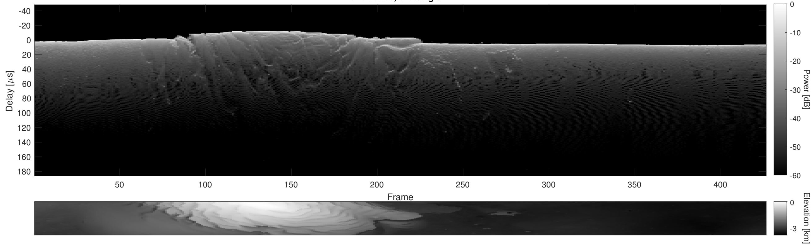
Orbit 5390, Cluttergram
