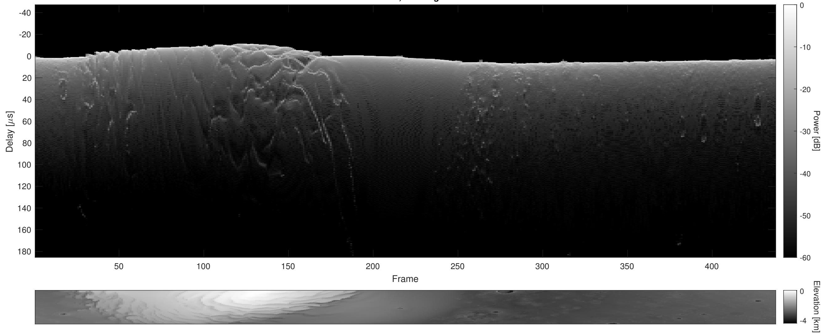
Orbit 5391, Cluttergram
