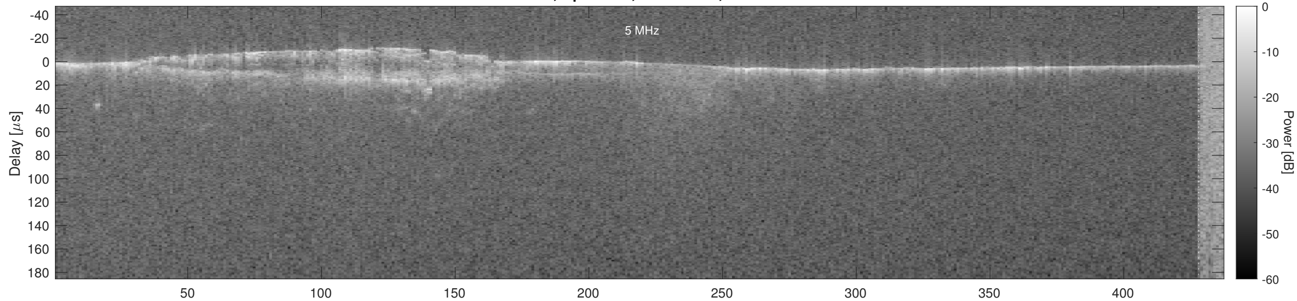
Orbit 5391, Optimized, No Window, Channel 2
