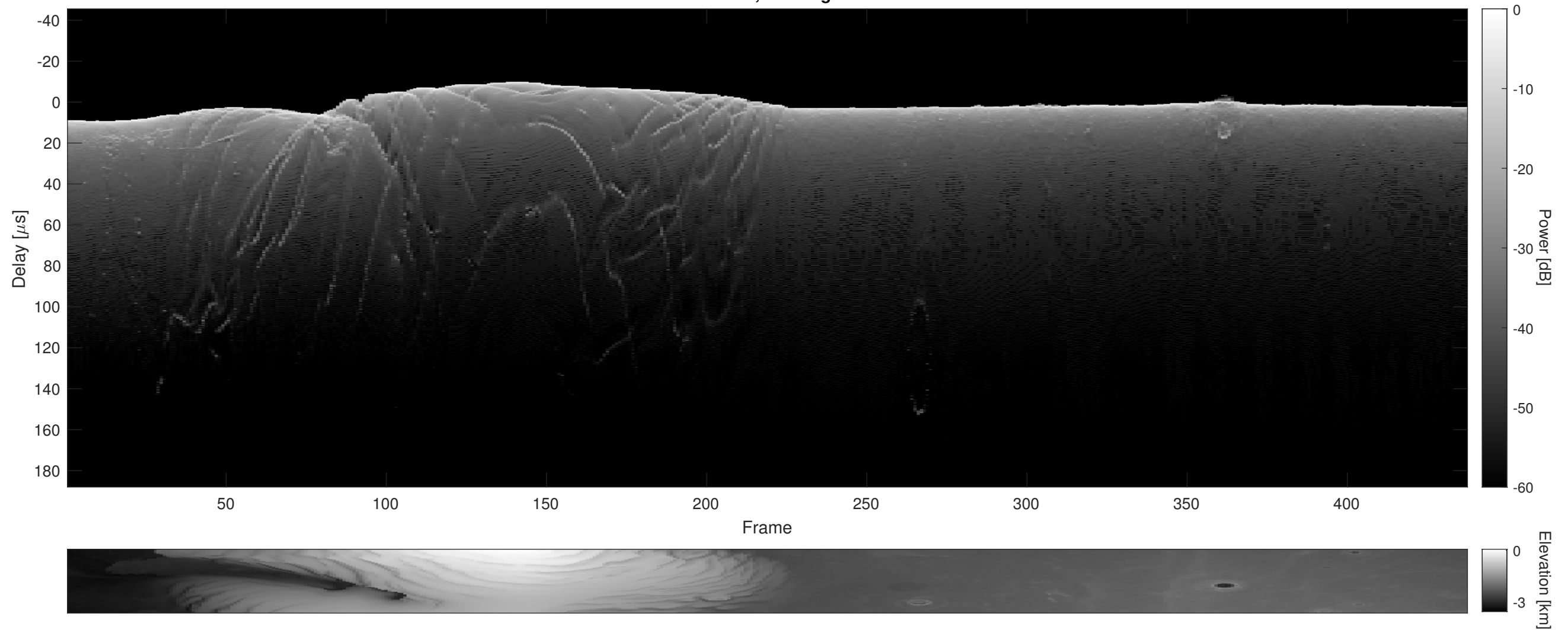
Orbit 5392, Cluttergram
