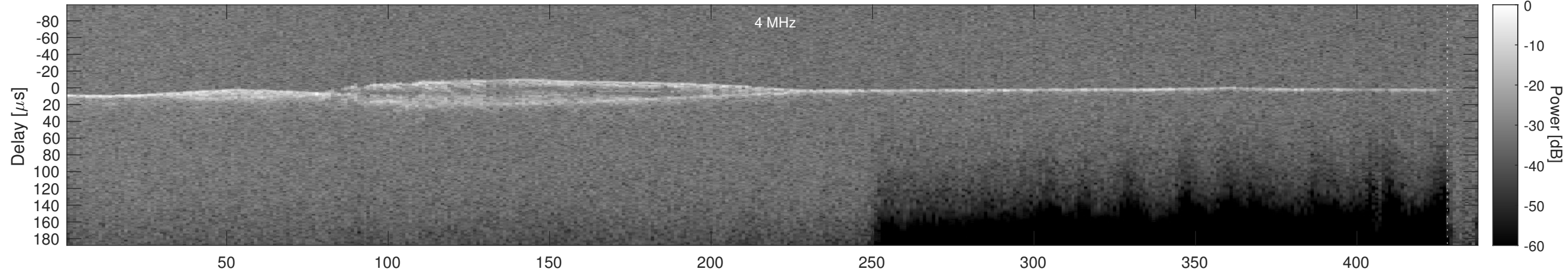
Orbit 5392, Cluttergram
