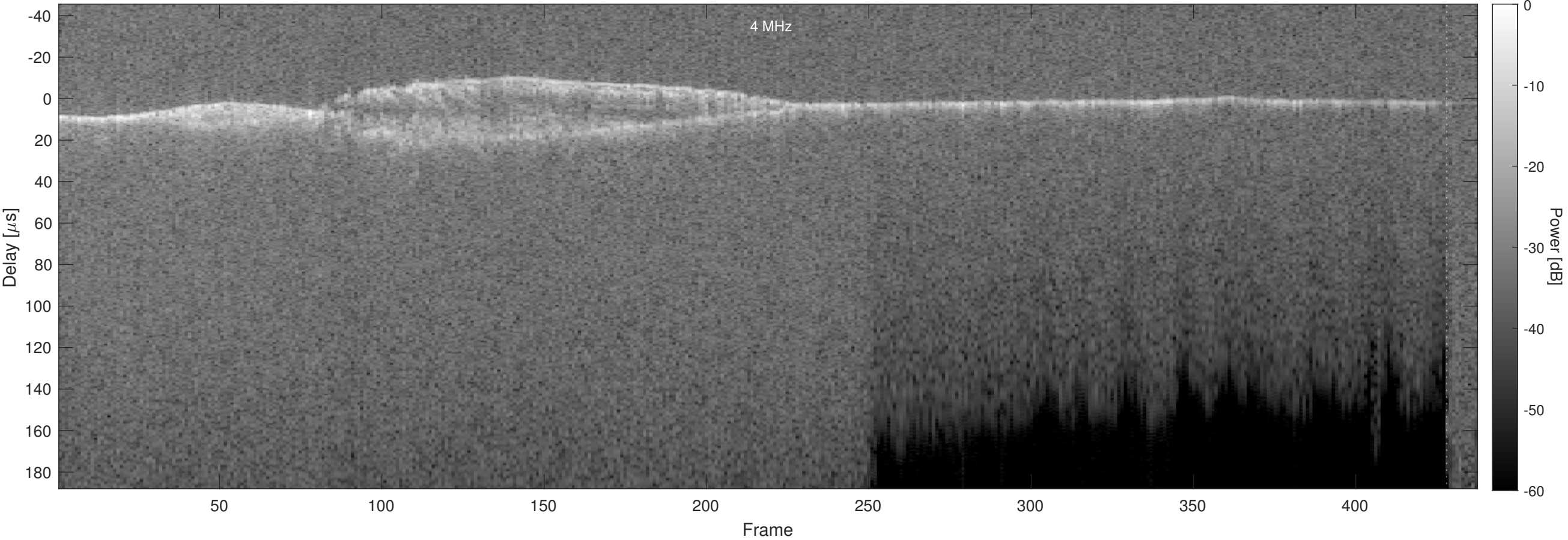
Orbit 5392, Optimized, No Window, Channel 2
