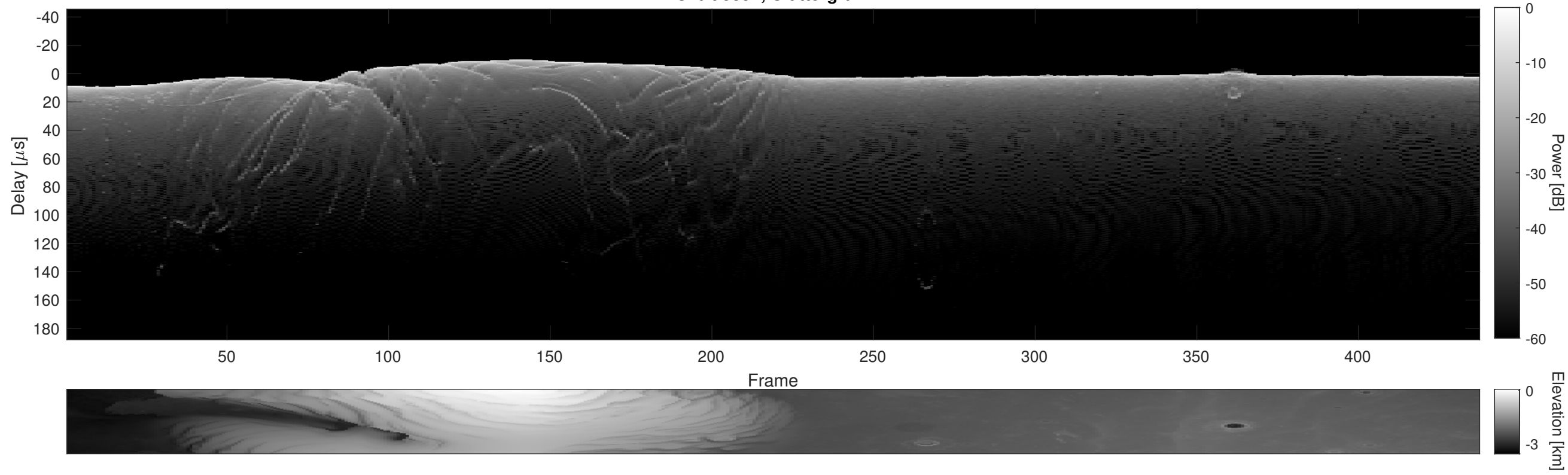
Orbit 5392, Cluttergram
