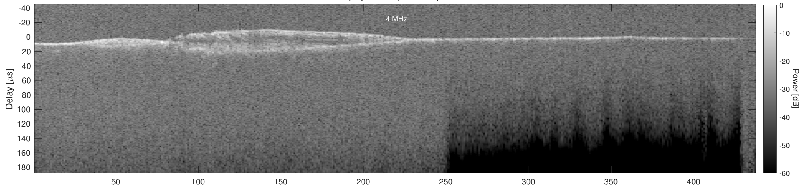
Orbit 5392, Cluttergram
