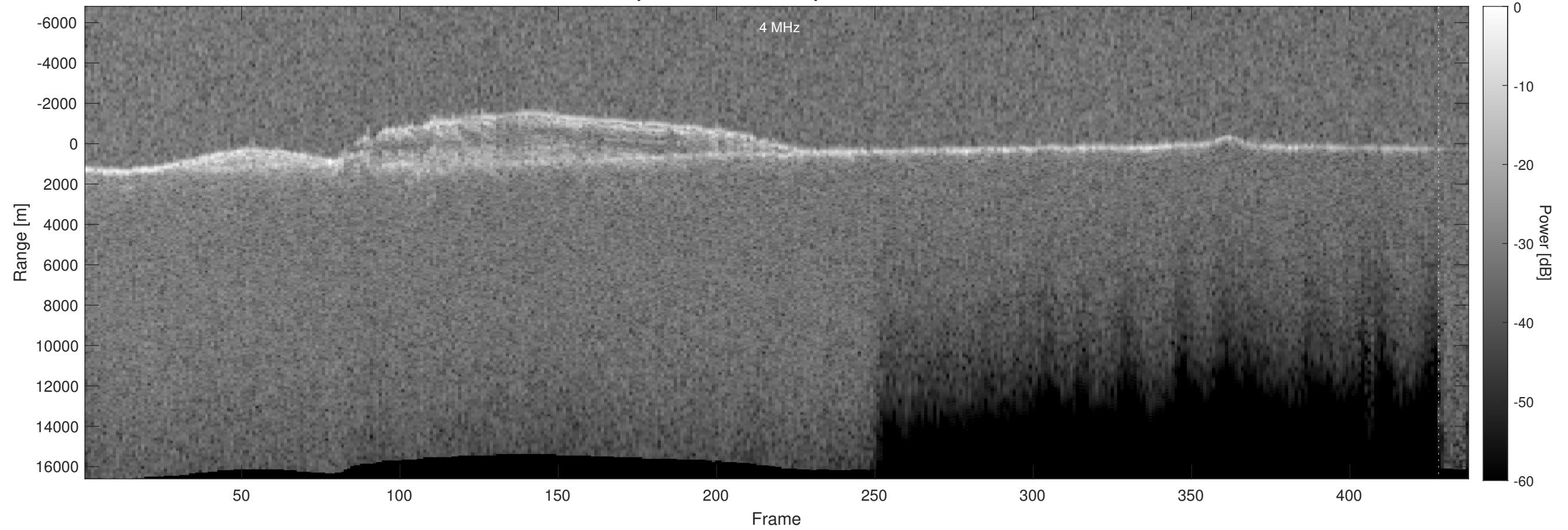
Orbit 5392, Optimized, Window, Depth-Corrected, Channel 2
