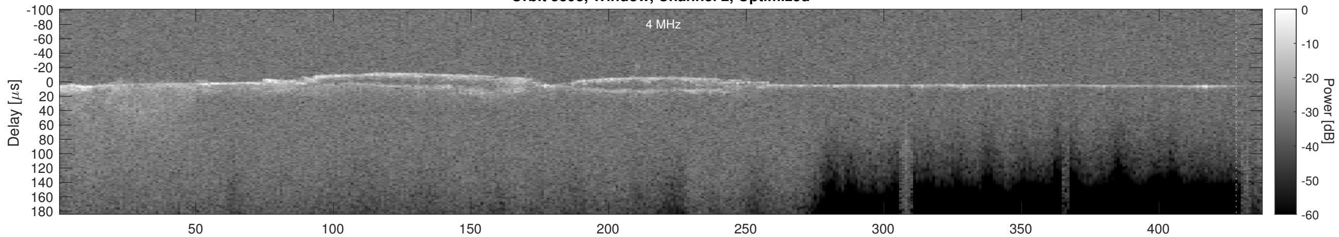
Orbit 5393, Cluttergram
