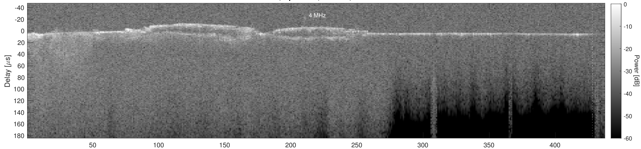
Orbit 5393, Cluttergram
