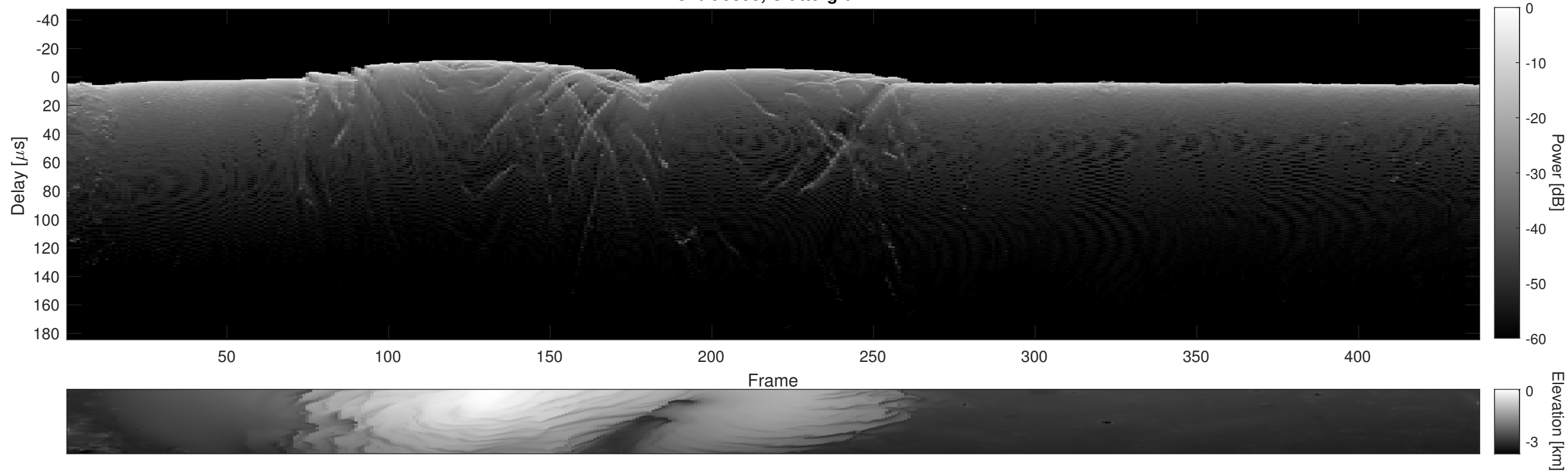
Orbit 5393, Cluttergram
