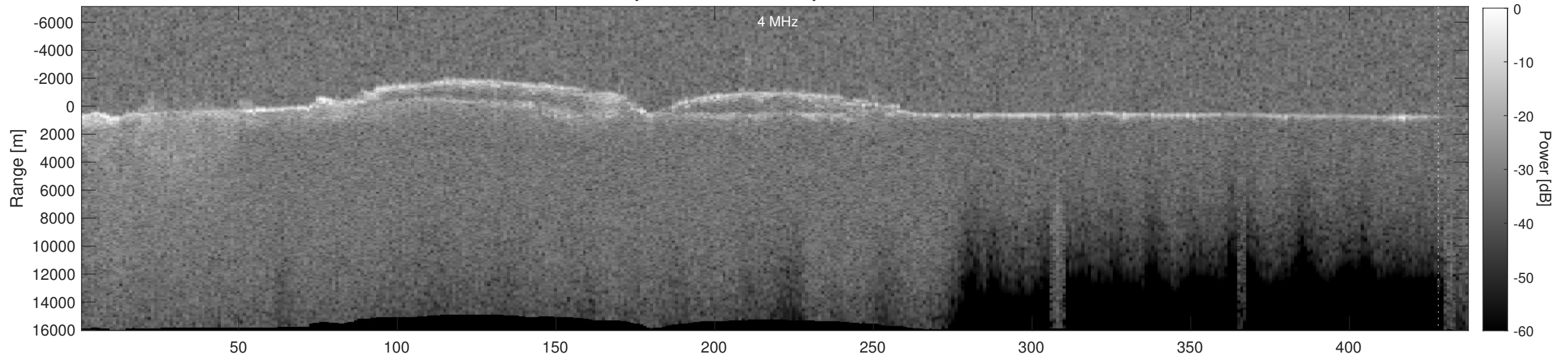
Orbit 5393, Depth-Corrected Cluttergram
