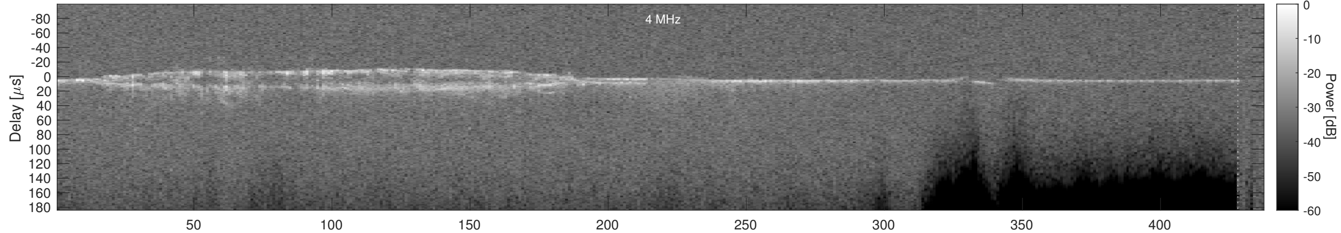
Orbit 5395, Cluttergram
