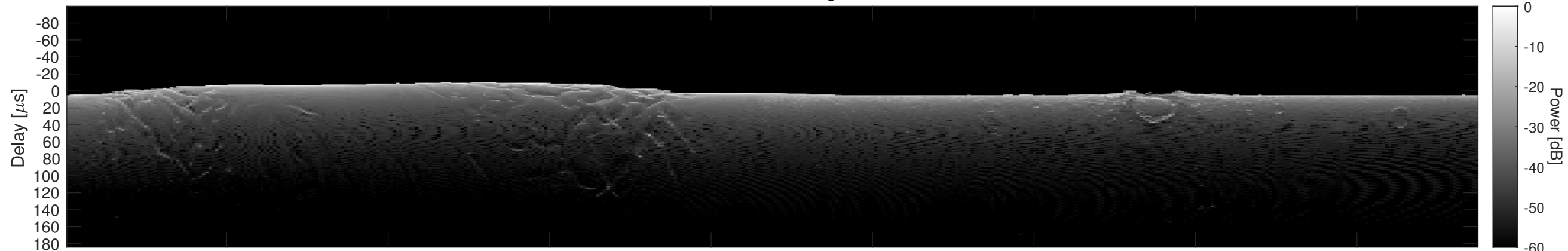
Orbit 5395, Cluttergram
