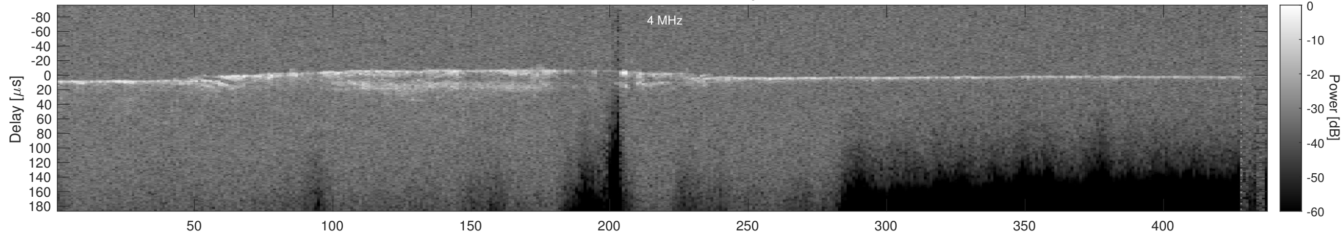
Orbit 5396, Cluttergram
