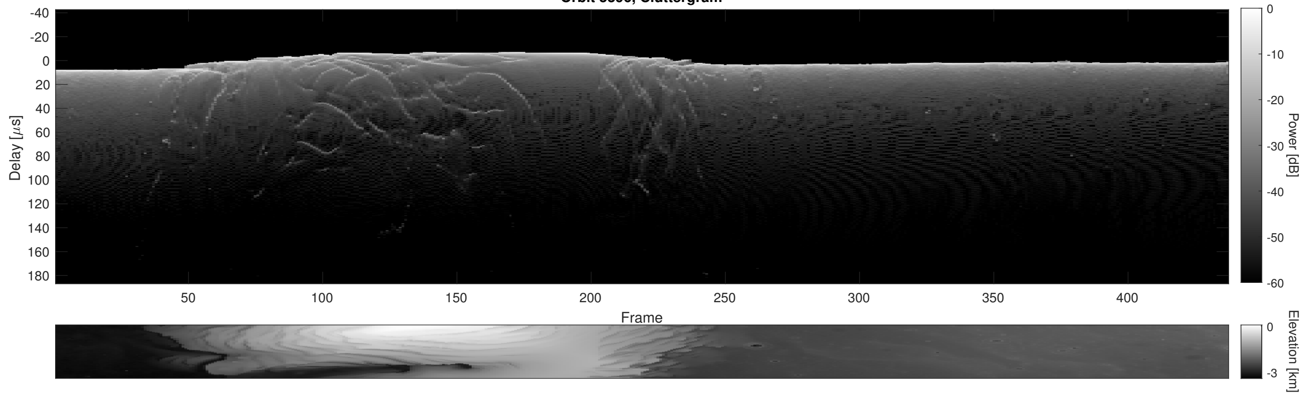
Orbit 5396, Cluttergram
