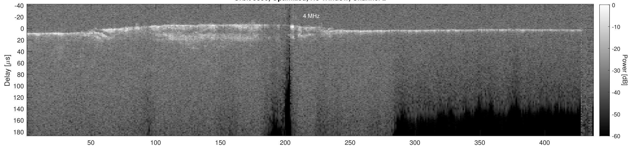
Orbit 5396, Cluttergram
