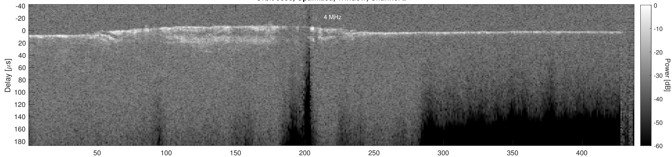
Orbit 5396, Cluttergram
