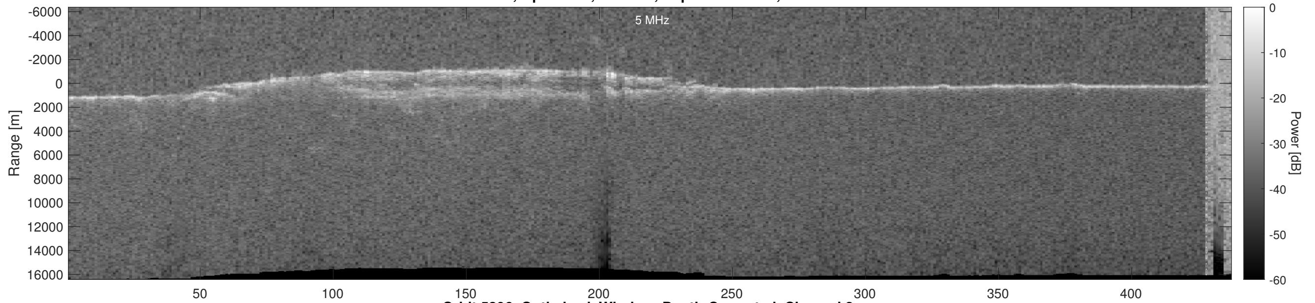
Orbit 5396, Optimized, Window, Depth-Corrected, Channel 2
