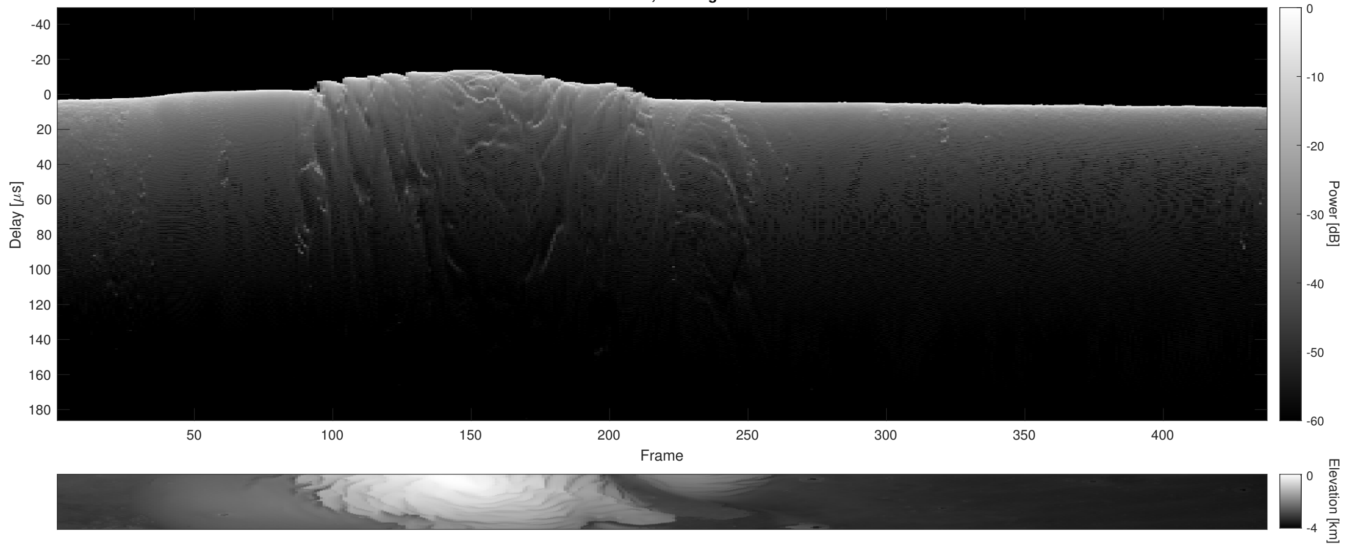
Orbit 5397, Cluttergram
