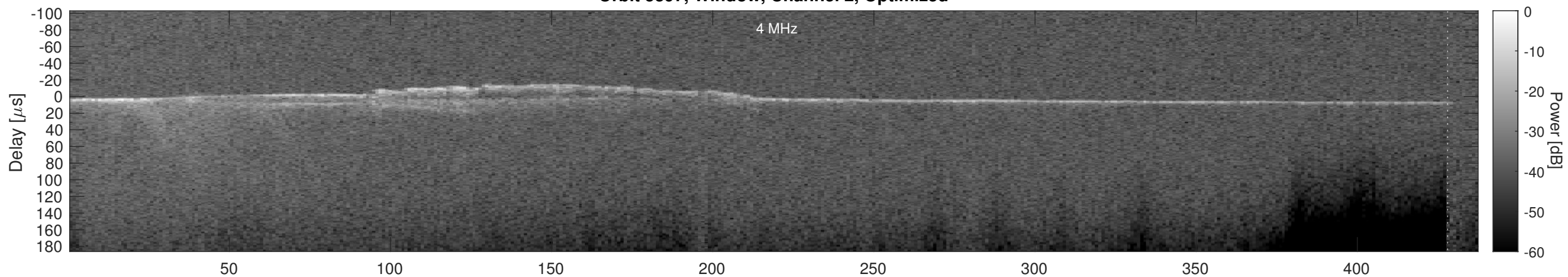
Orbit 5397, Cluttergram
