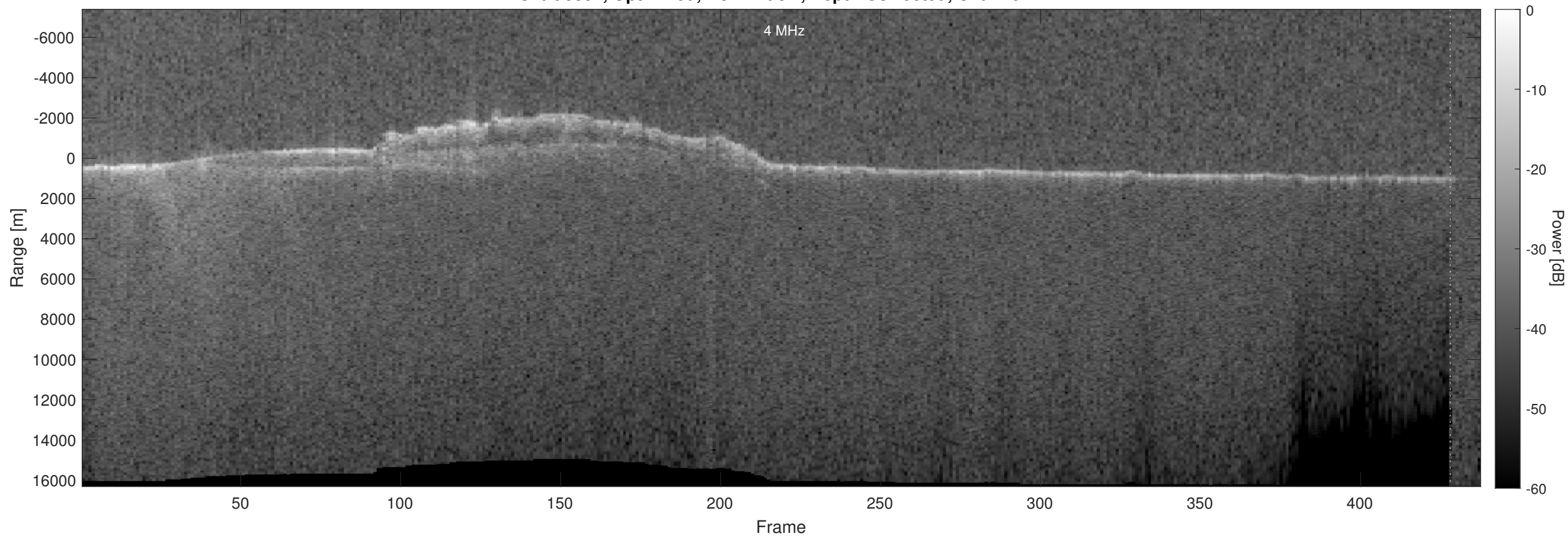
Orbit 5397, Optimized, No Window, Depth-Corrected, Channel 2
