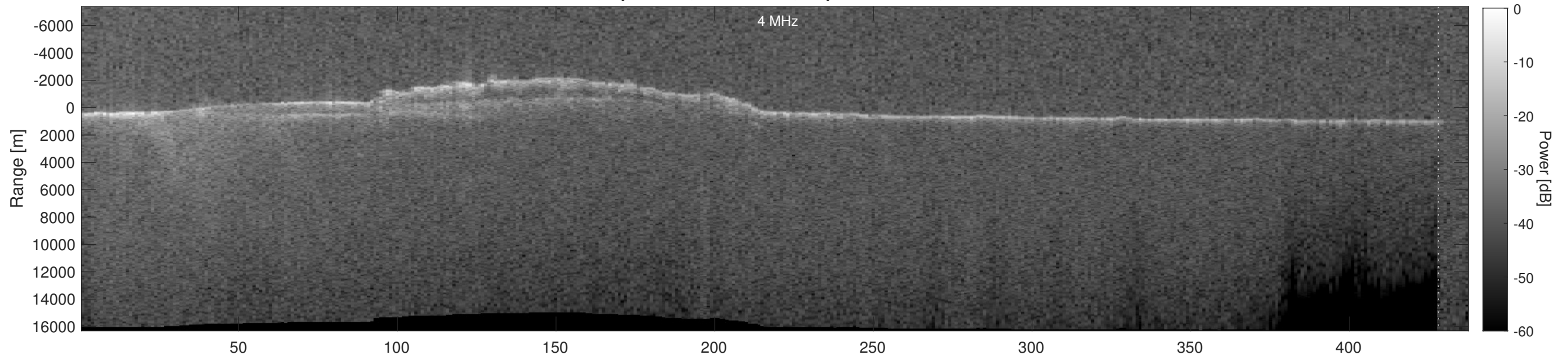
Orbit 5397, Depth-Corrected Cluttergram
