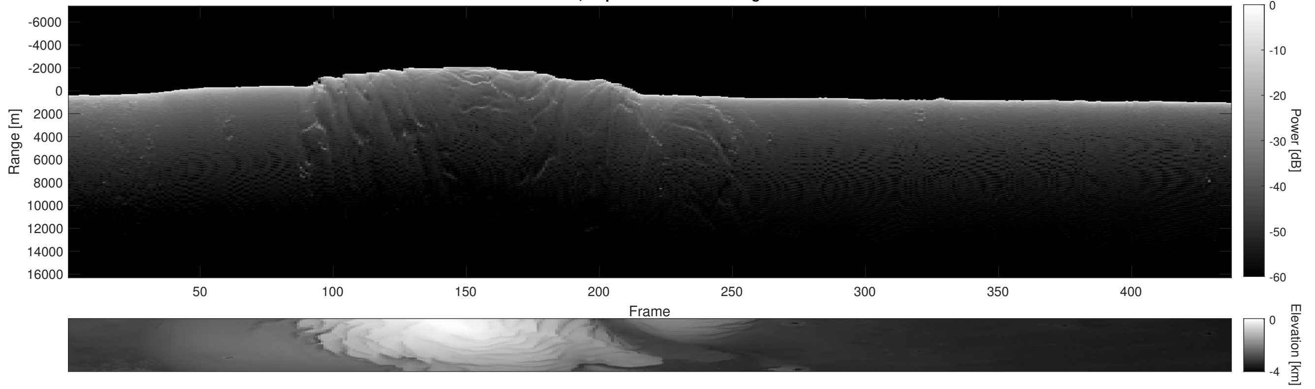
Orbit 5397, Depth-Corrected Cluttergram
