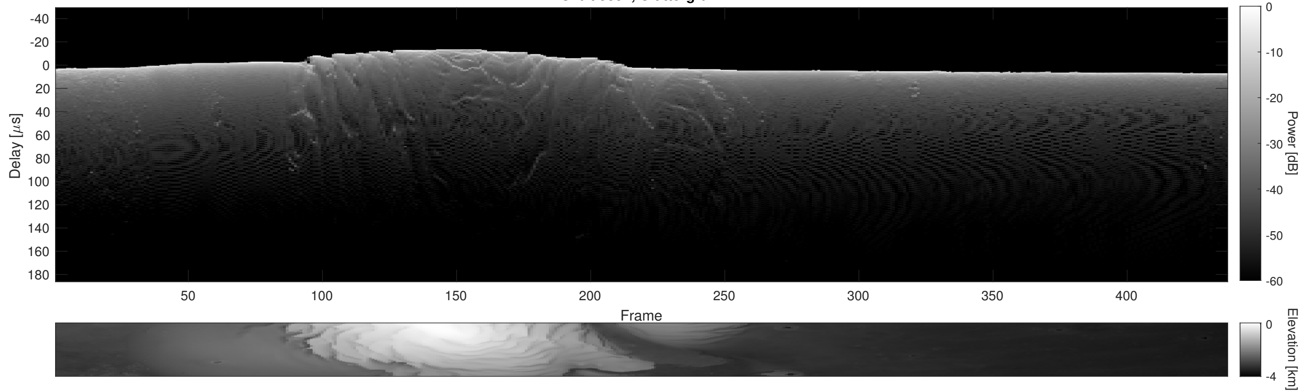
Orbit 5397, Cluttergram
