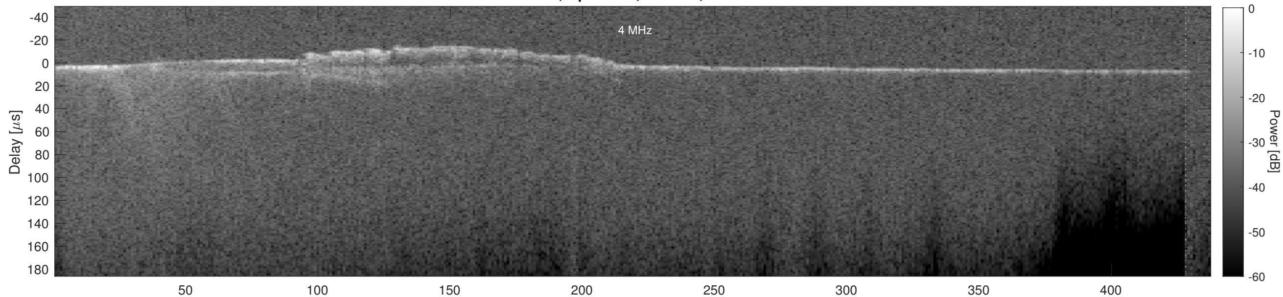
Orbit 5397, Cluttergram
