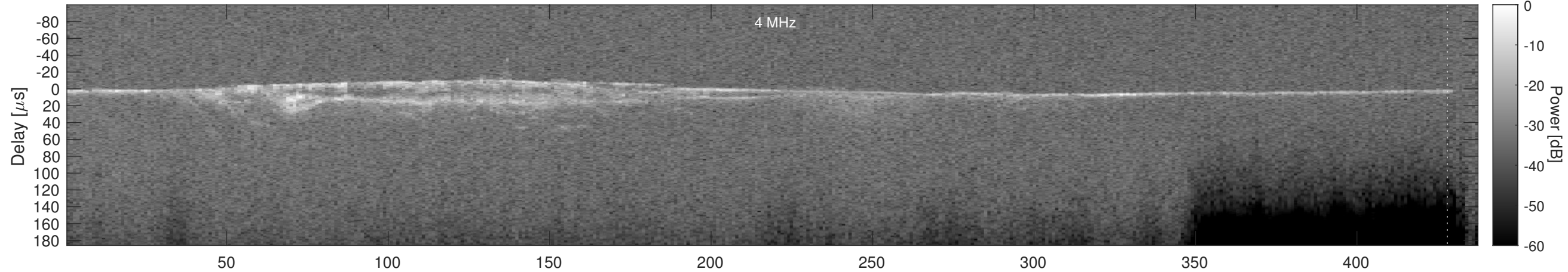
Orbit 5398, Cluttergram
