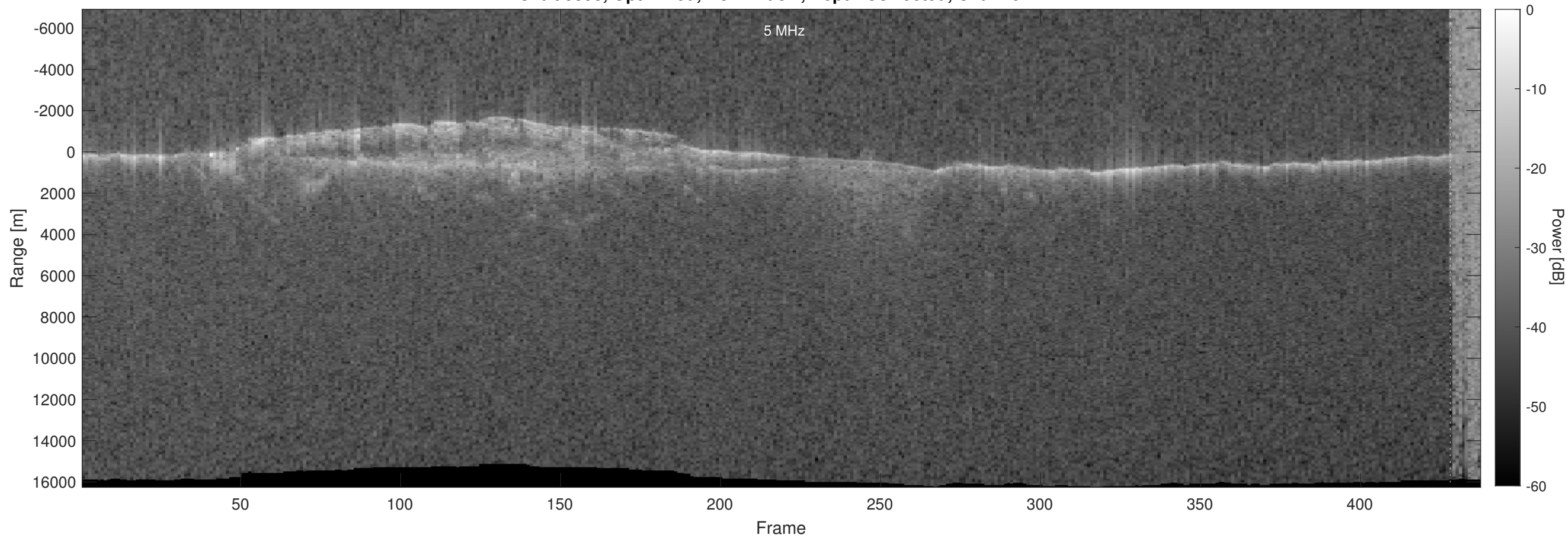
Orbit 5398, Optimized, No Window, Depth-Corrected, Channel 2
