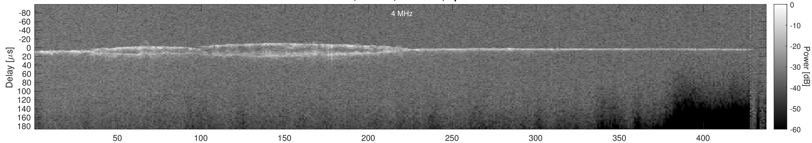
Orbit 5399, Cluttergram
