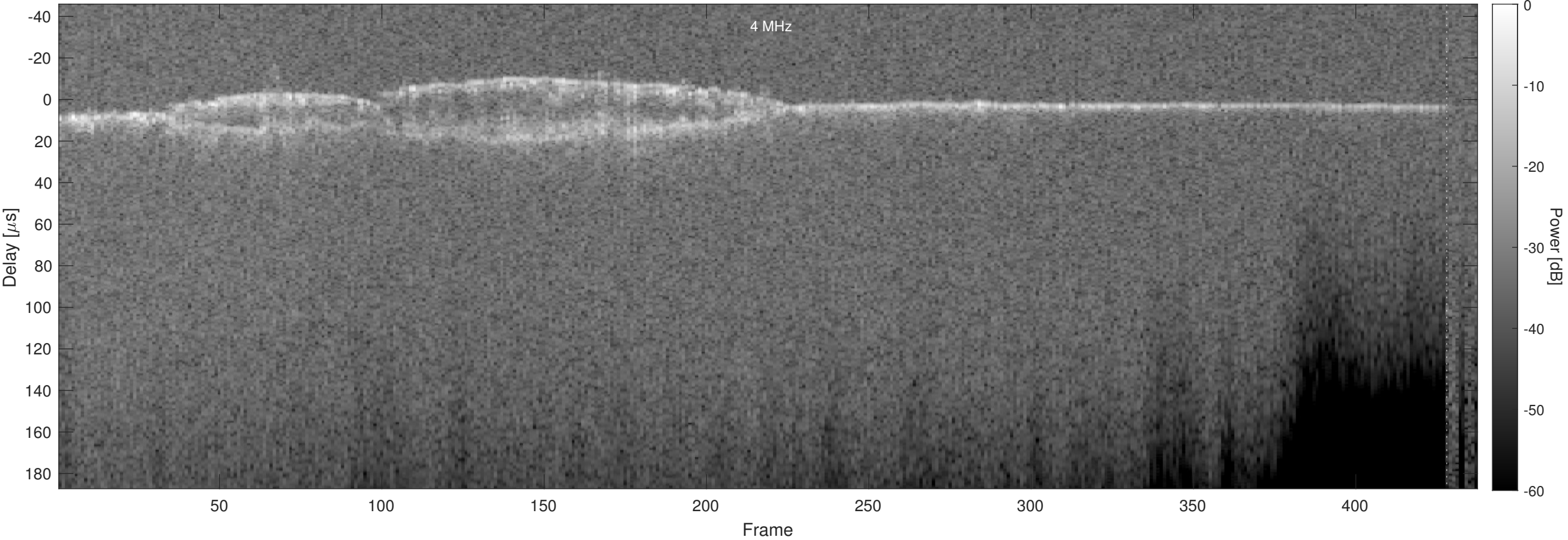
Orbit 5399, Optimized, Window, Channel 2
