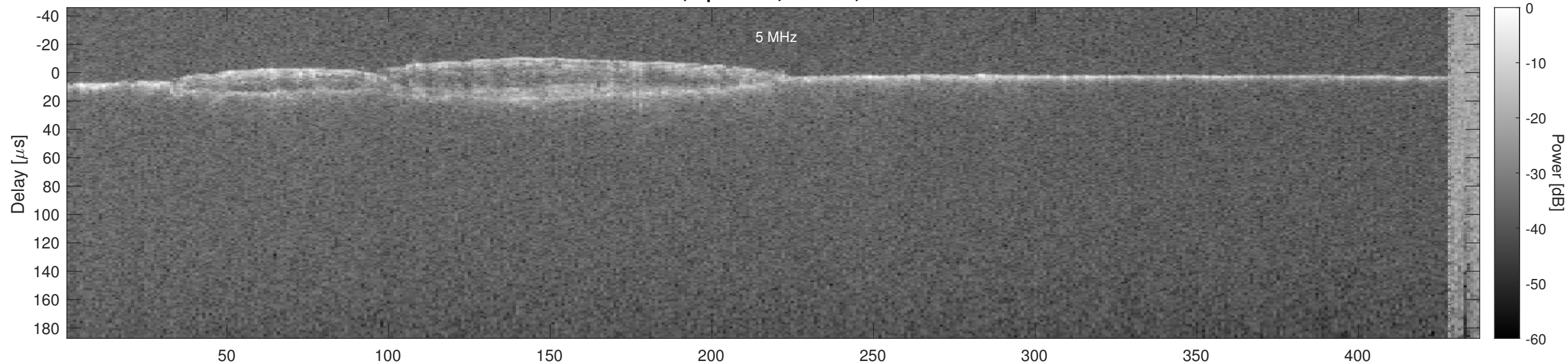
Orbit 5399, Optimized, Window, Channel 2
