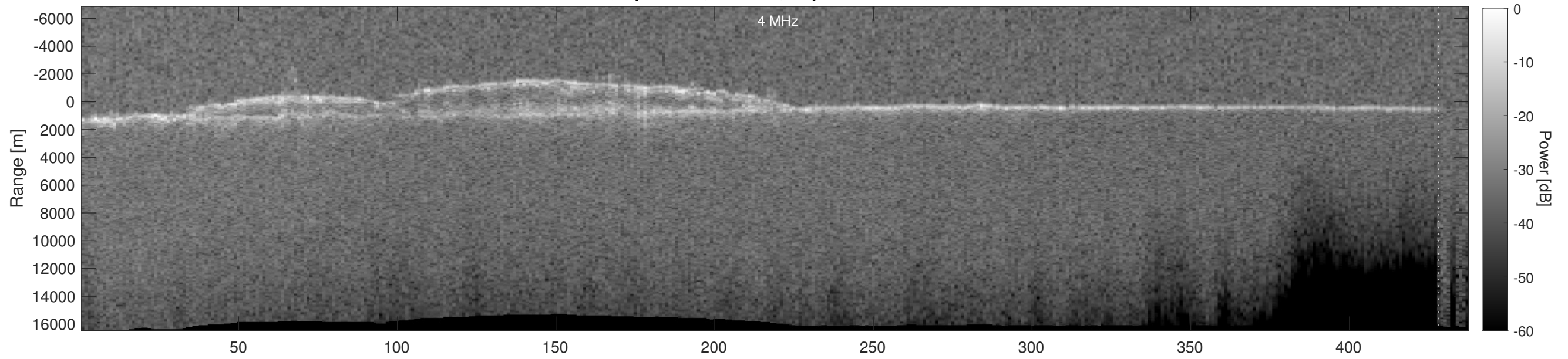
Orbit 5399, Depth-Corrected Cluttergram
