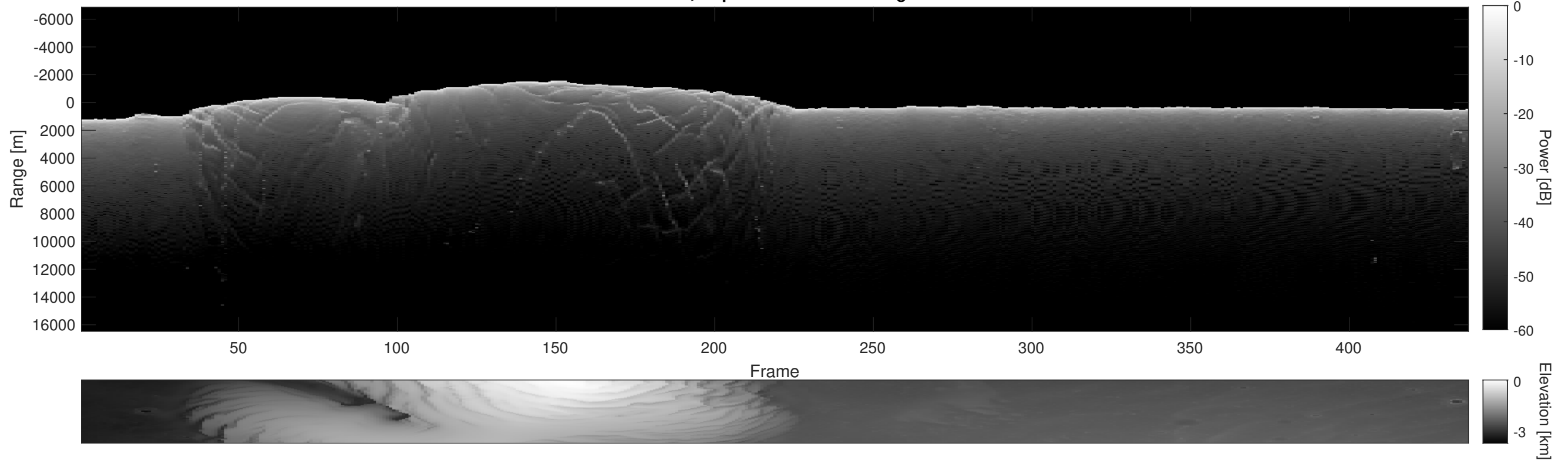
Orbit 5399, Depth-Corrected Cluttergram
