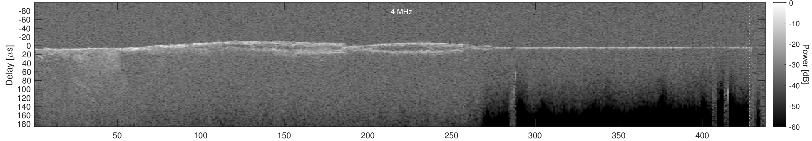
Orbit 5400, Cluttergram
