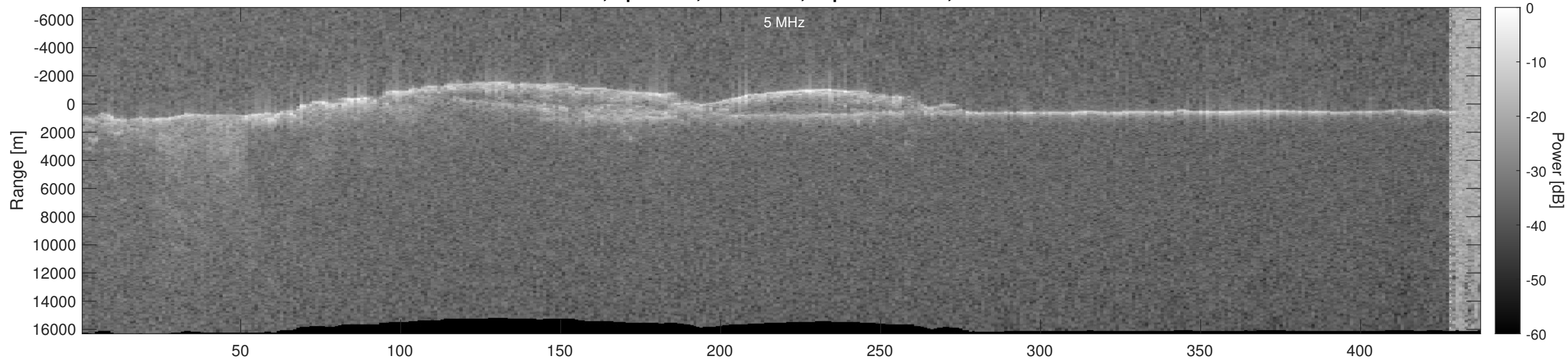
Orbit 5400, Optimized, No Window, Depth-Corrected, Channel 2
