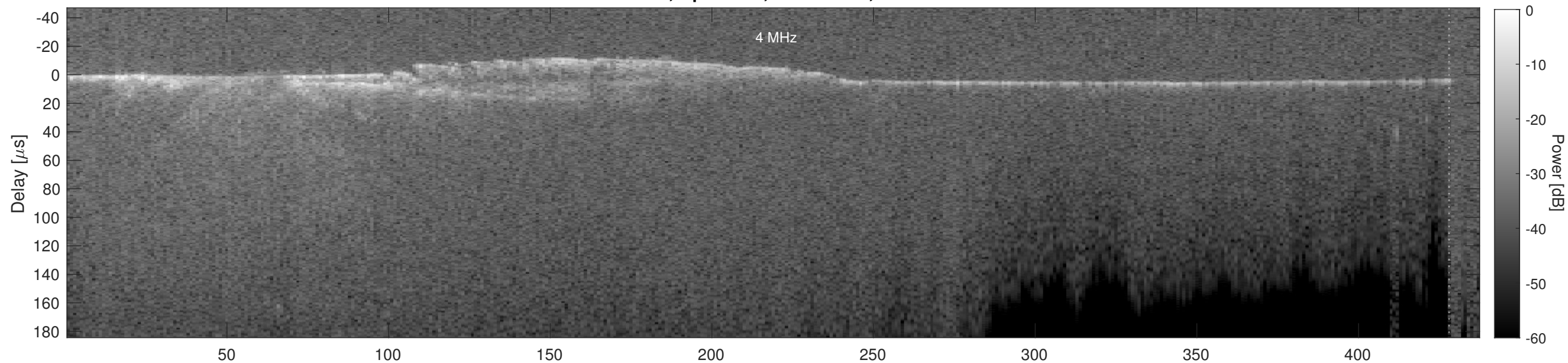
Orbit 5401, Cluttergram
