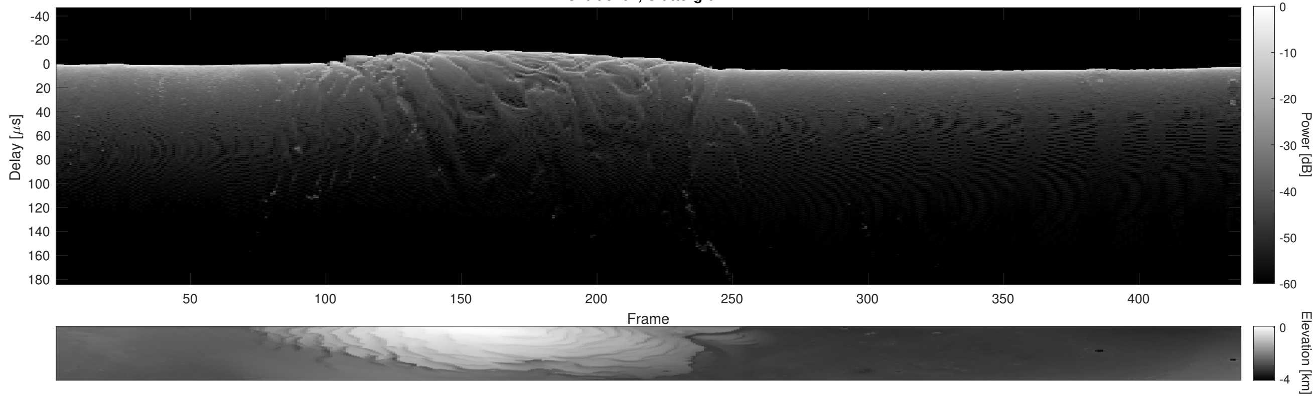
Orbit 5401, Cluttergram
